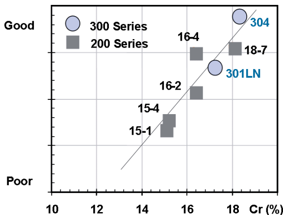
Chromium content influence
