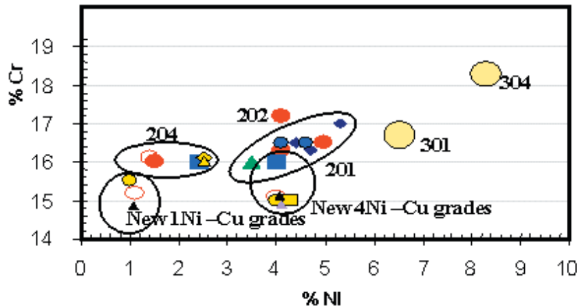
Nickel/chrome balance in austenitic grades
